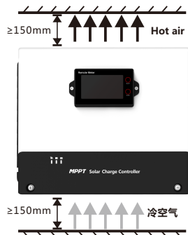
Fig. 2.1 Installation and Heat Dissipation
