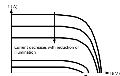
Fig.1-3 Relation Between Solar Battery Output Characteristics and Illumination
